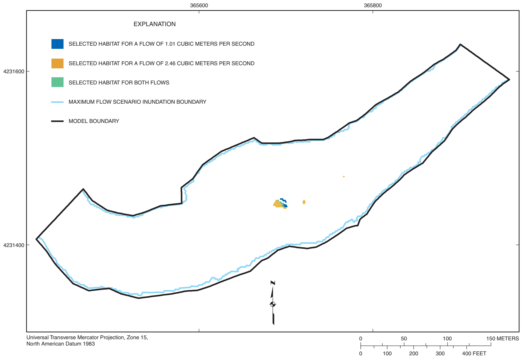
Figure 4-68. Selected habitat area distribution for habitat category 19 (stonecat) at flows of 1.01 and 2.46 cubic meters per second at Marais des Cygnes River site MDC2.
